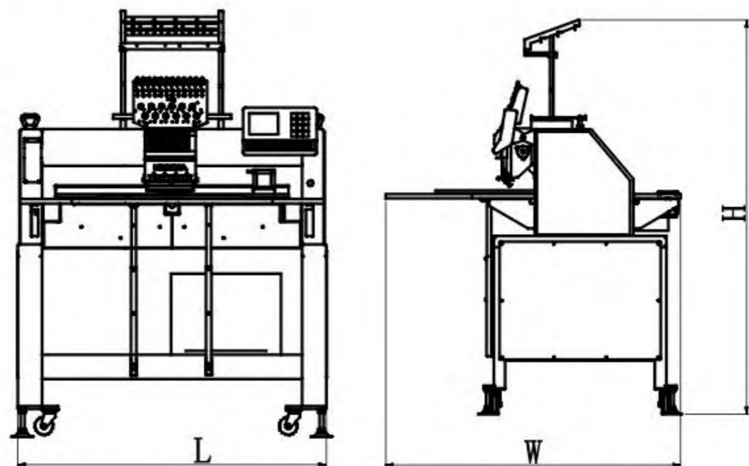
RCM-1201C X450Y450 L:1260 W:1300 H:1740 (mm)
